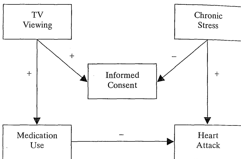
Figure 1: Diagram indicating causal influences among variables in example scenario illustrating selection bias due to informed consent. Plus sign indicates positive influence; minus sign indicates negative influence.
